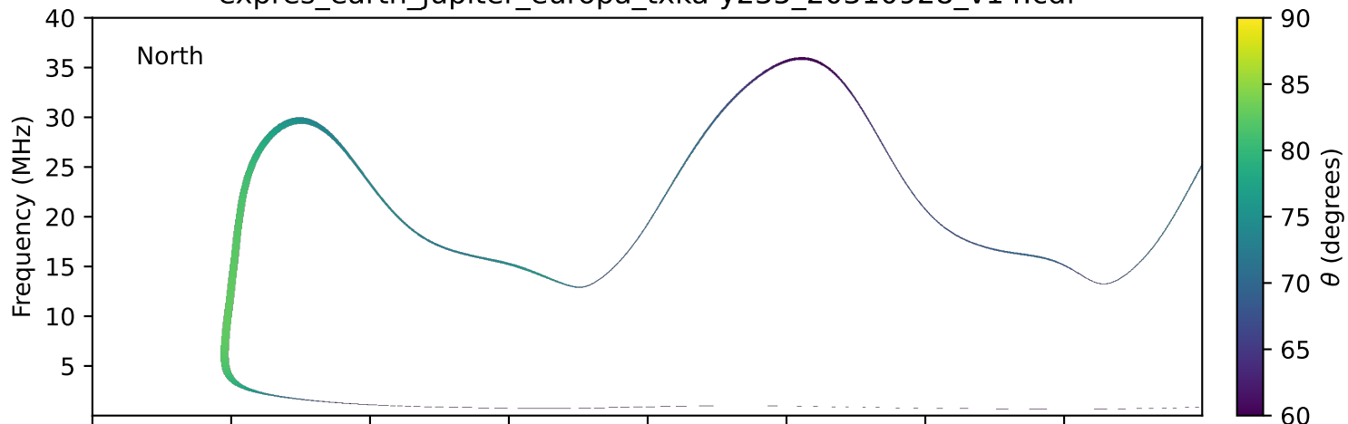
expres_earth_jupiter_europa_txka-y235_20310928_v14.cdf
