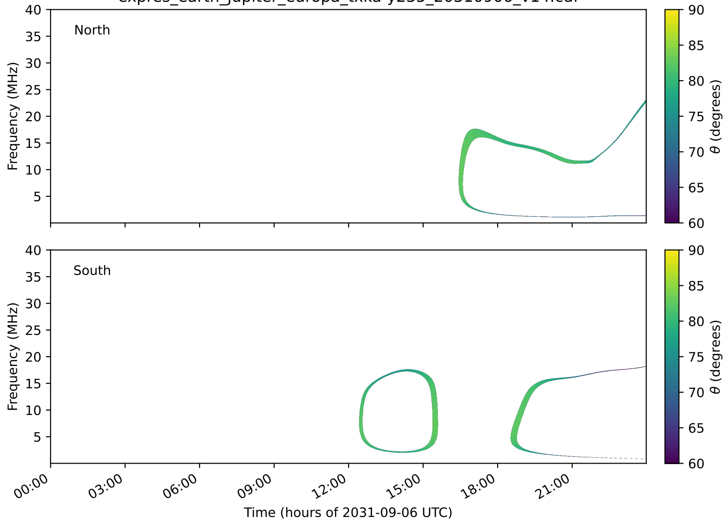
expres_earth_jupiter_europa_txka-y235_20310906_v14.cdf
