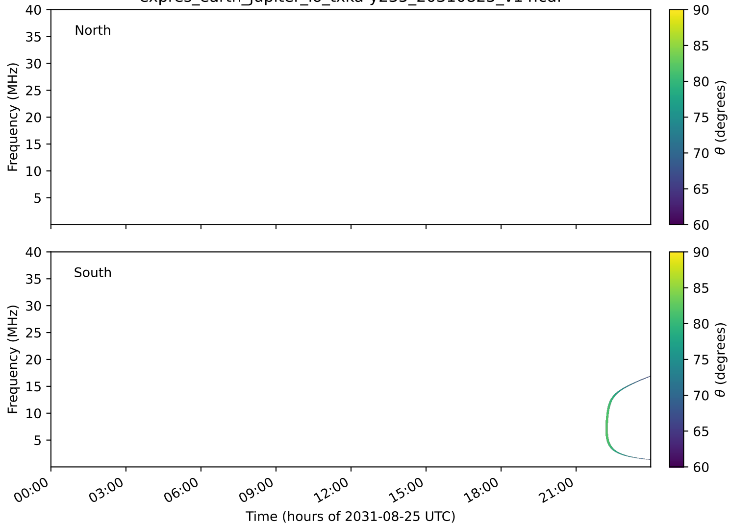
expres_earth_jupiter_io_txka-y235_20310825_v14.cdf
