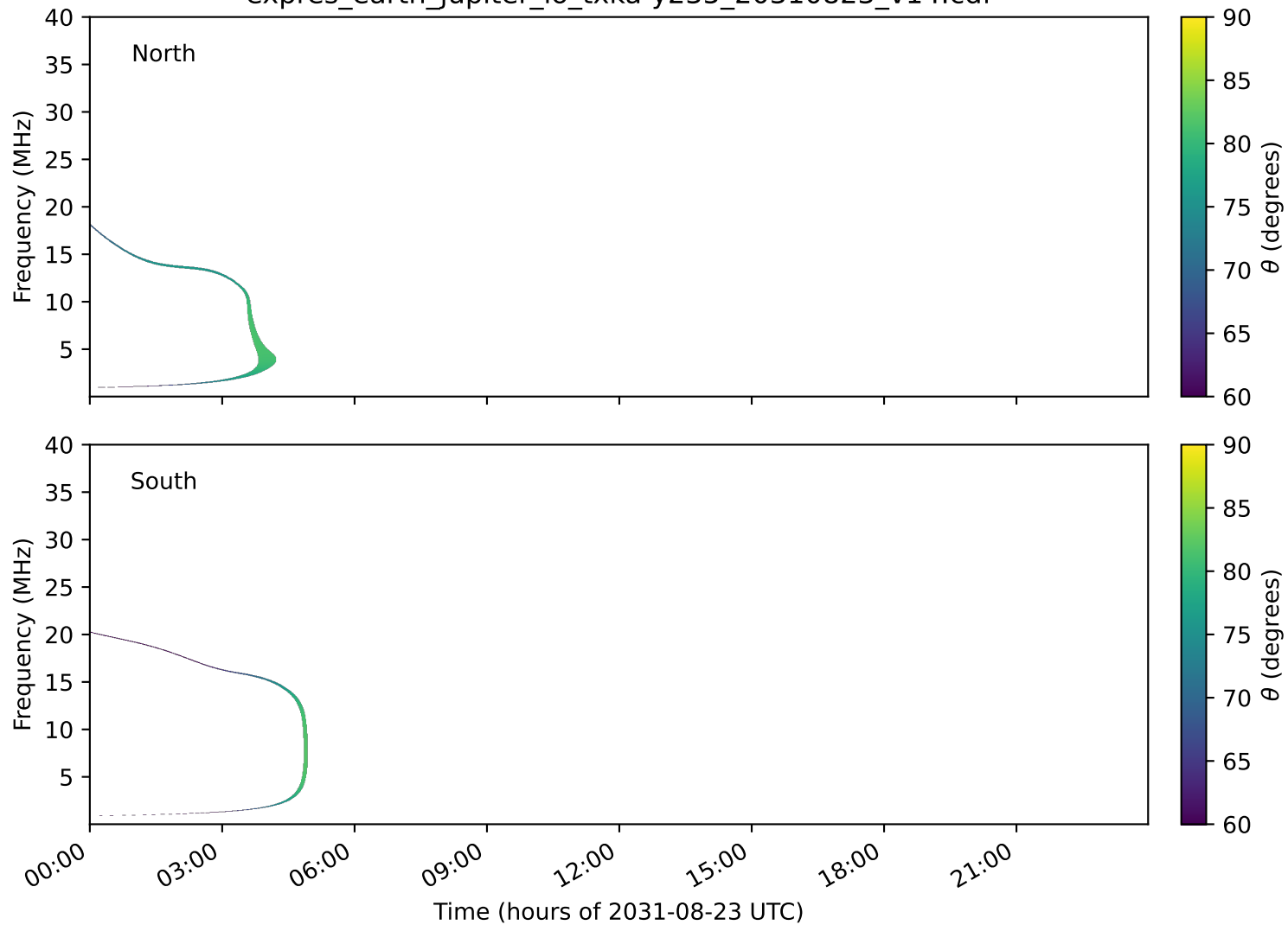
expres_earth_jupiter_io_txka-y235_20310823_v14.cdf
