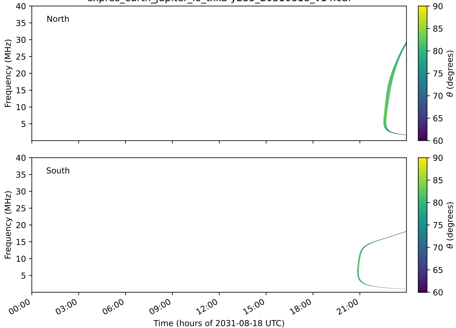
expres_earth_jupiter_io_txka-y235_20310818_v14.cdf
