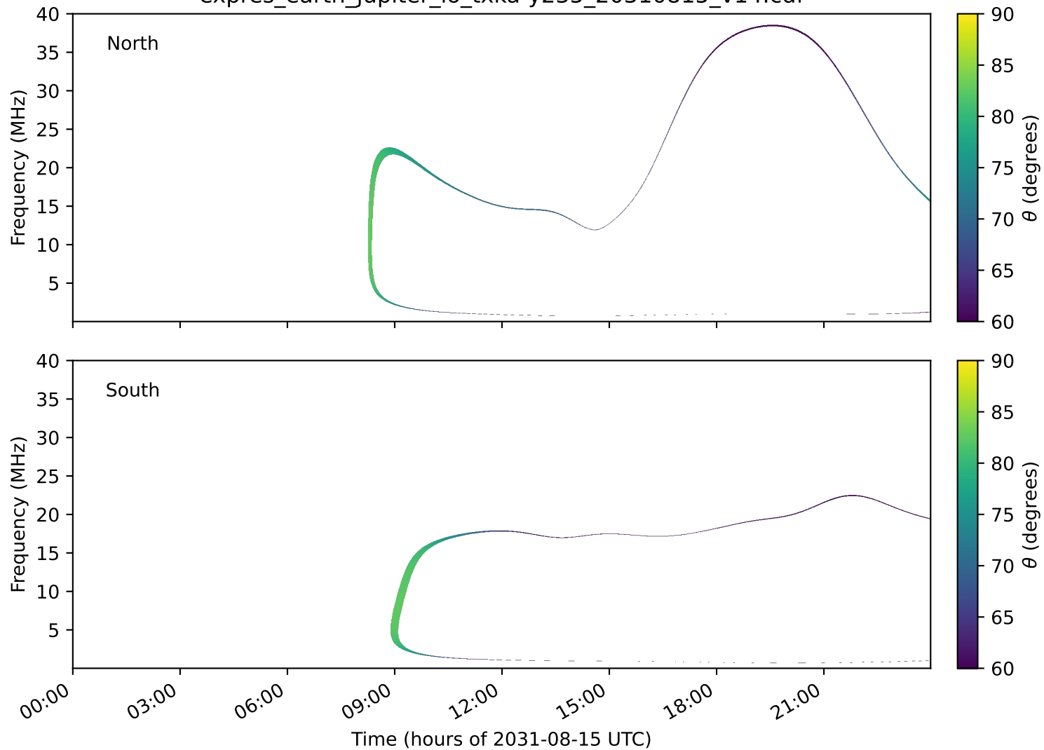
expres_earth_jupiter_io_txka-y235_20310815_v14.cdf
