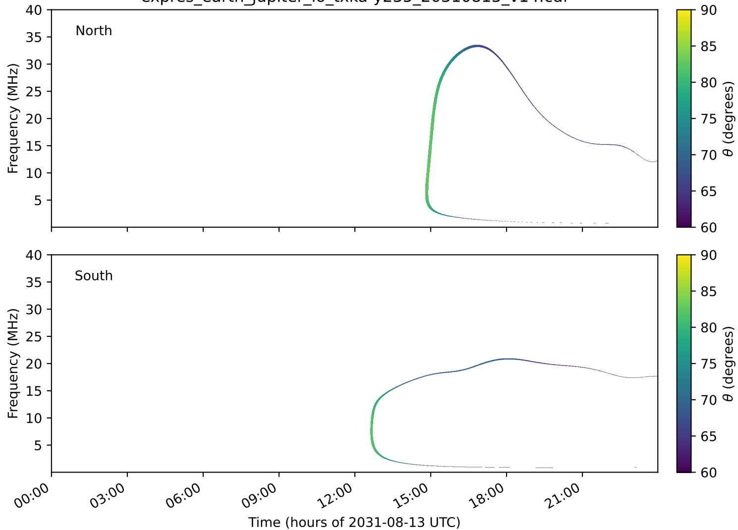
expres_earth_jupiter_io_txka-y235_20310813_v14.cdf
