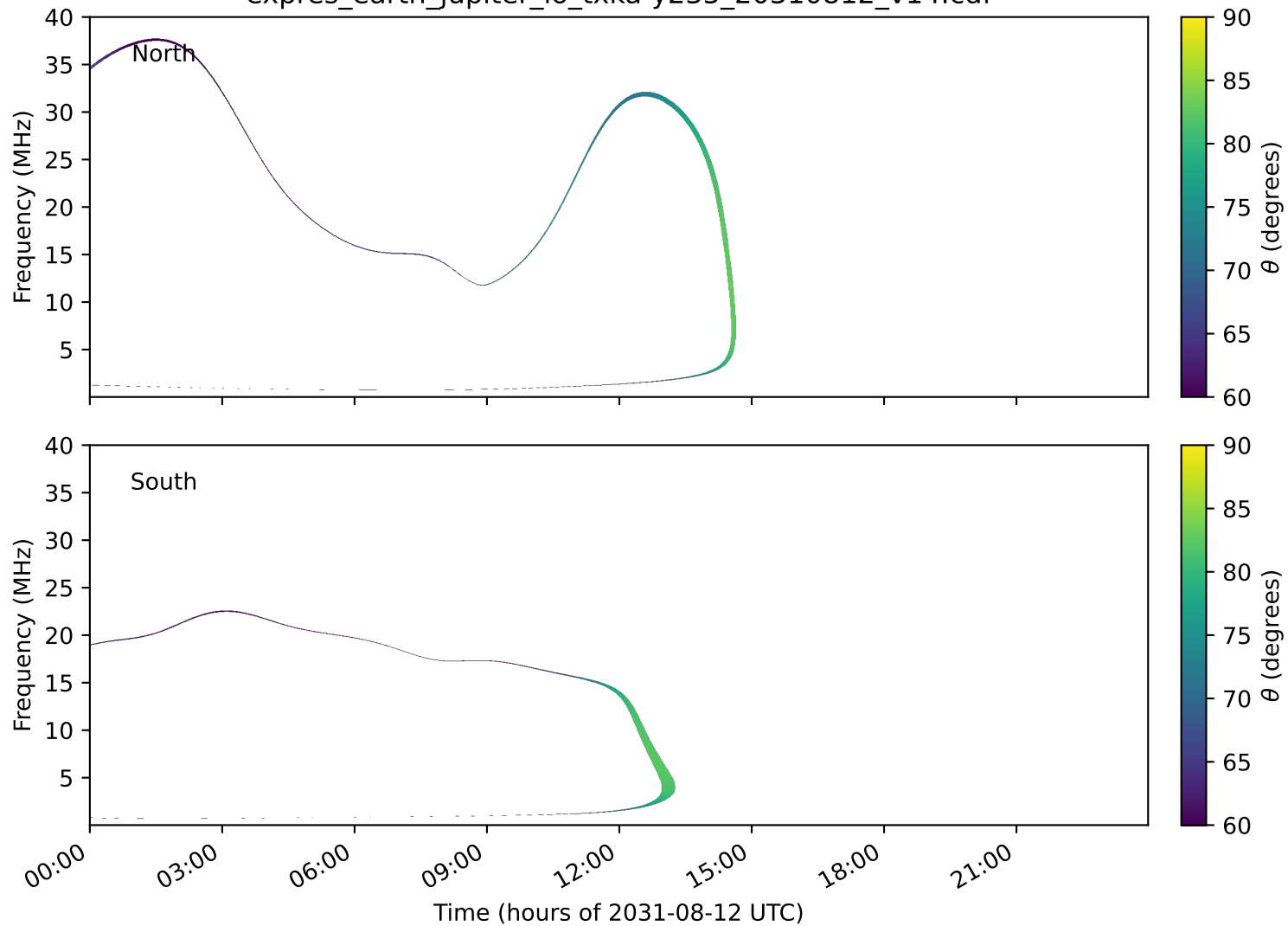
expres_earth_jupiter_io_txka-y235_20310812_v14.cdf
