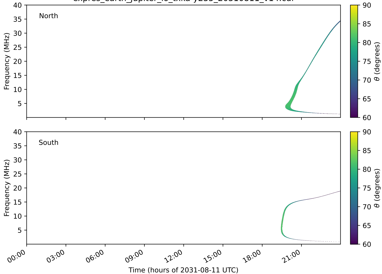
expres_earth_jupiter_io_txka-y235_20310811_v14.cdf
