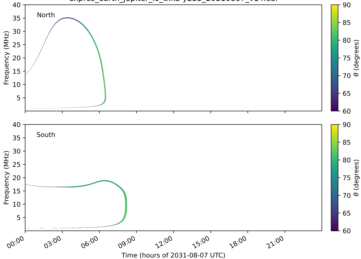
expres_earth_jupiter_io_txka-y235_20310807_v14.cdf
