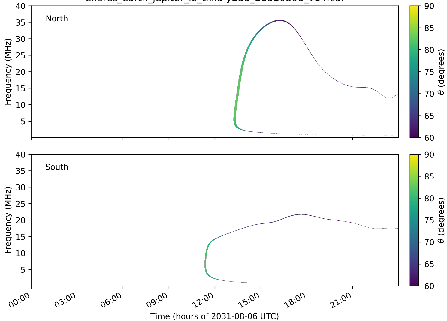
expres_earth_jupiter_io_txka-y235_20310806_v14.cdf
