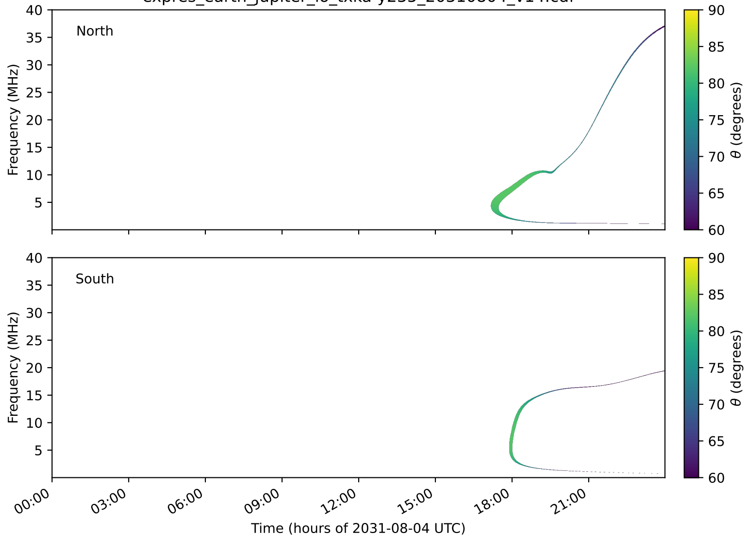
expres_earth_jupiter_io_txka-y235_20310804_v14.cdf
