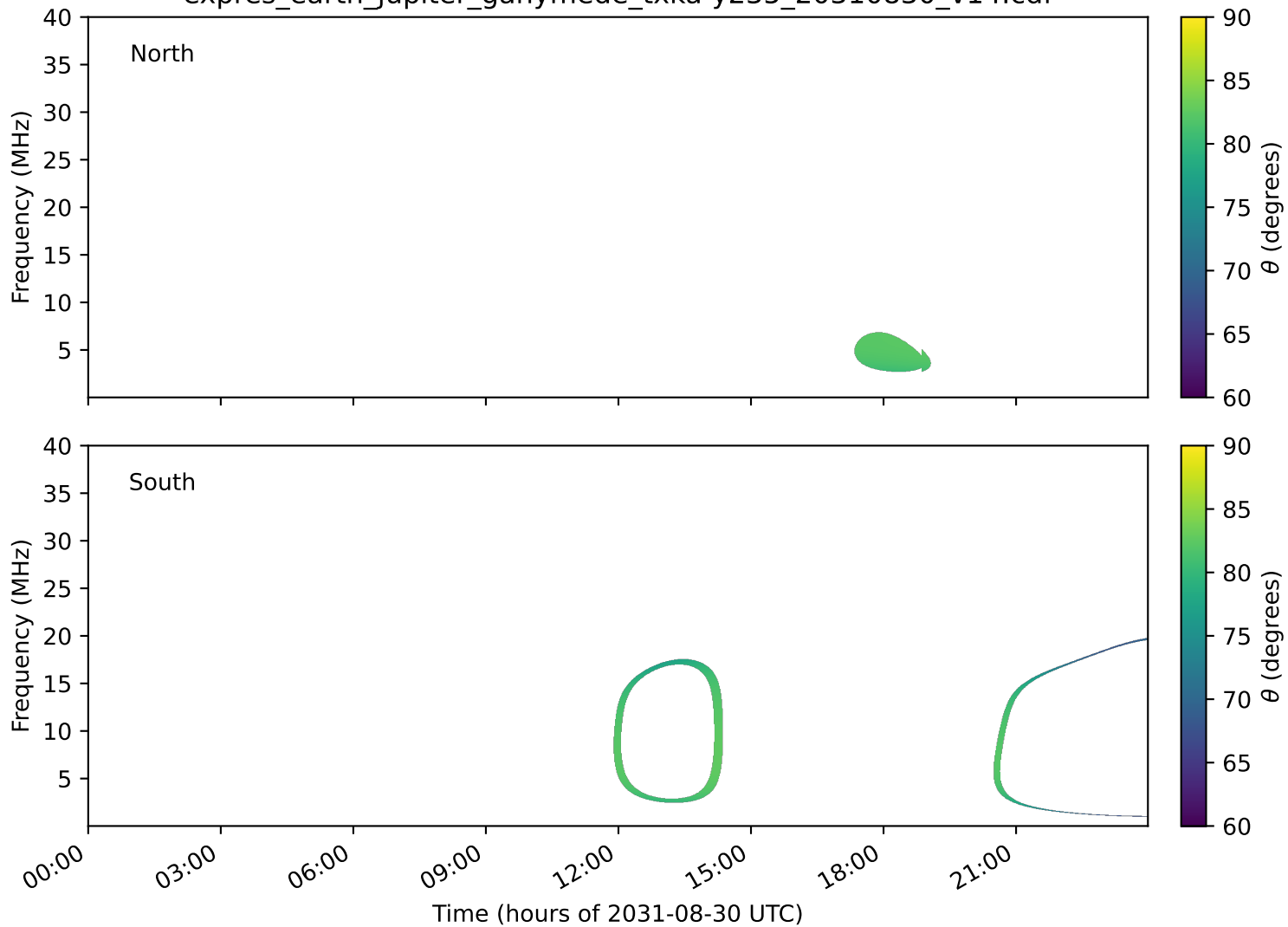
expres_earth_jupiter_ganymede_txka-y235_20310830_v14.cdf
