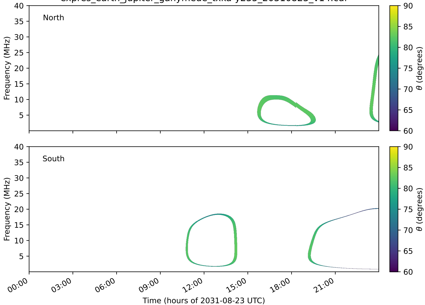
expres_earth_jupiter_ganymede_txka-y235_20310823_v14.cdf
