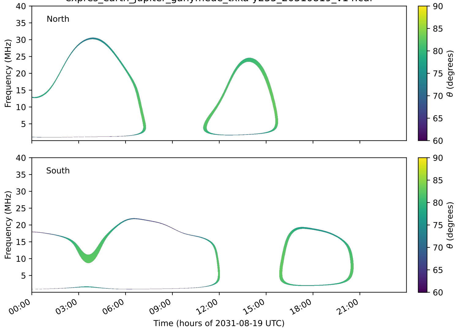
expres_earth_jupiter_ganymede_txka-y235_20310819_v14.cdf
