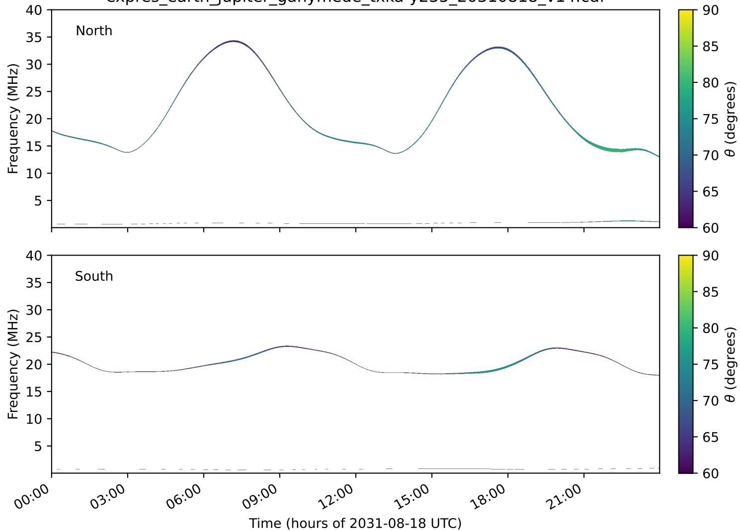
expres_earth_jupiter_ganymede_txka-y235_20310818_v14.cdf
