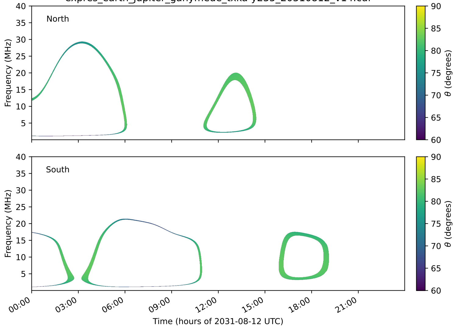
expres_earth_jupiter_ganymede_txka-y235_20310812_v14.cdf
