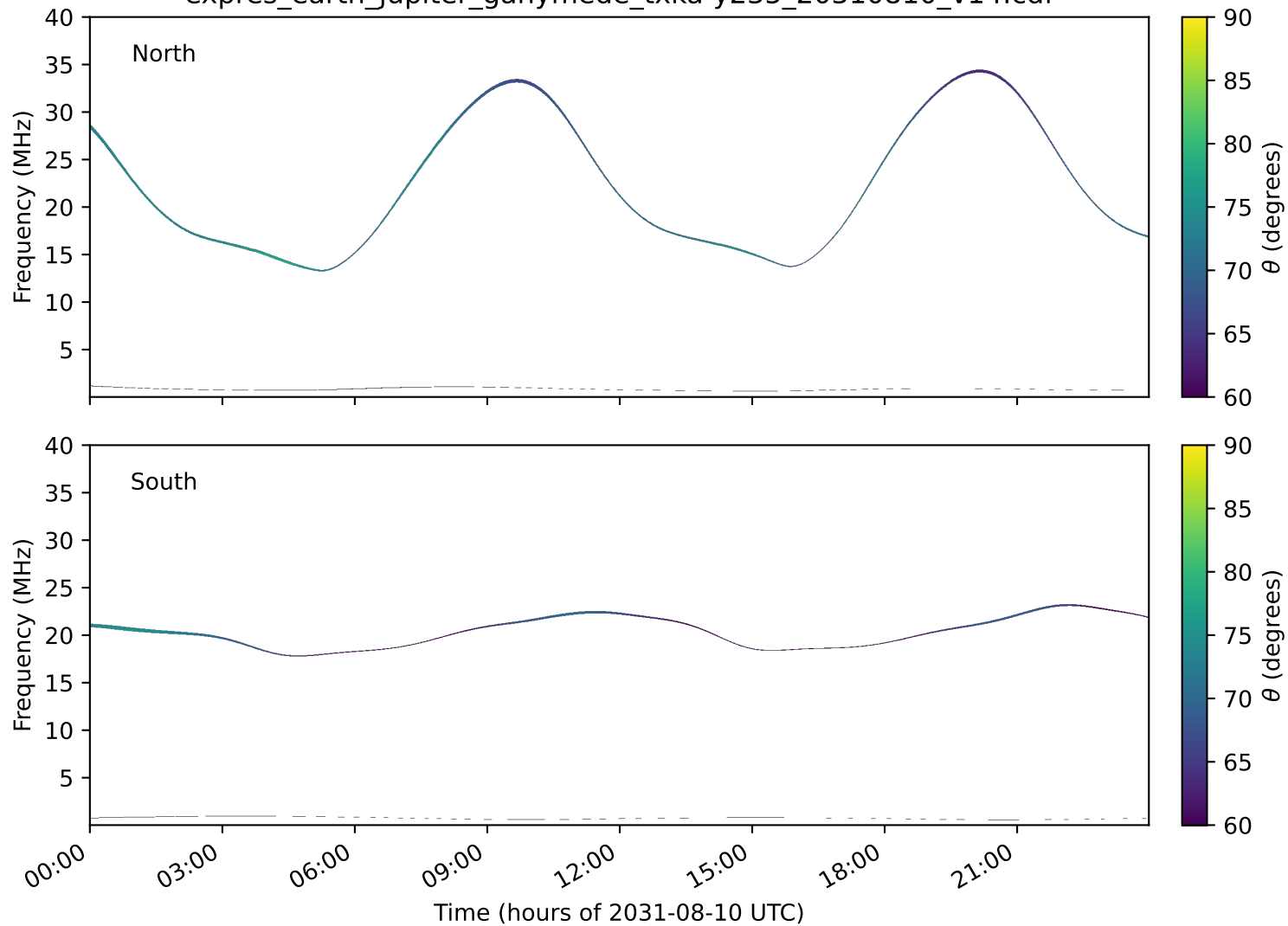
expres_earth_jupiter_ganymede_txka-y235_20310810_v14.cdf
