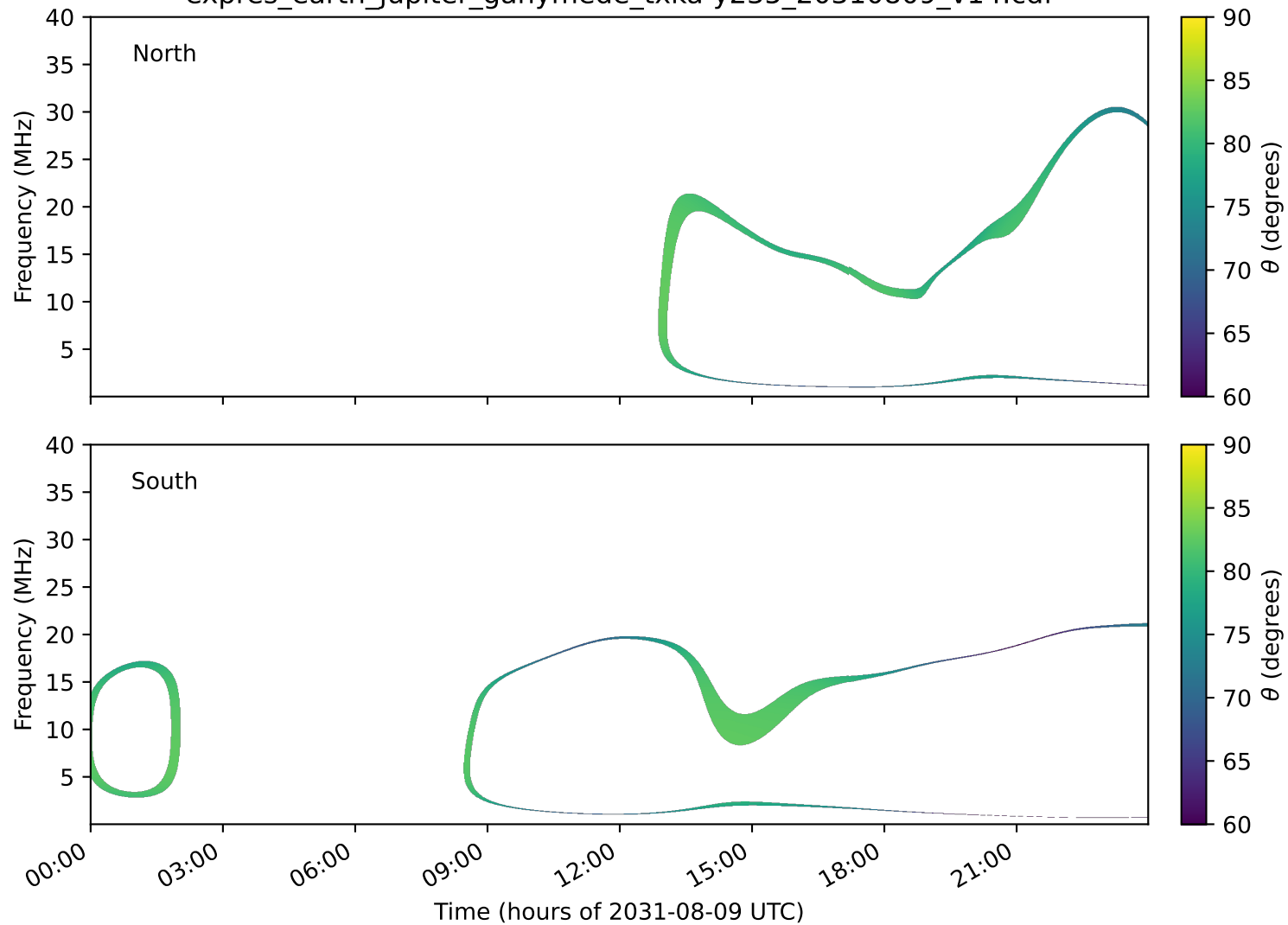
expres_earth_jupiter_ganymede_txka-y235_20310809_v14.cdf
