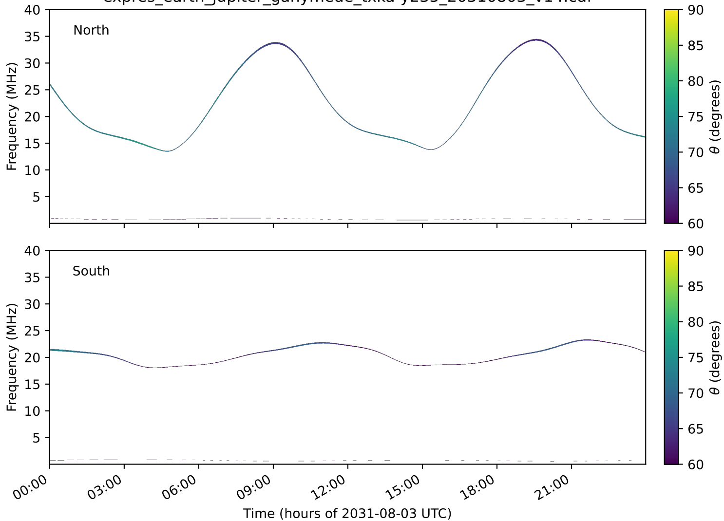
expres_earth_jupiter_ganymede_txka-y235_20310803_v14.cdf
