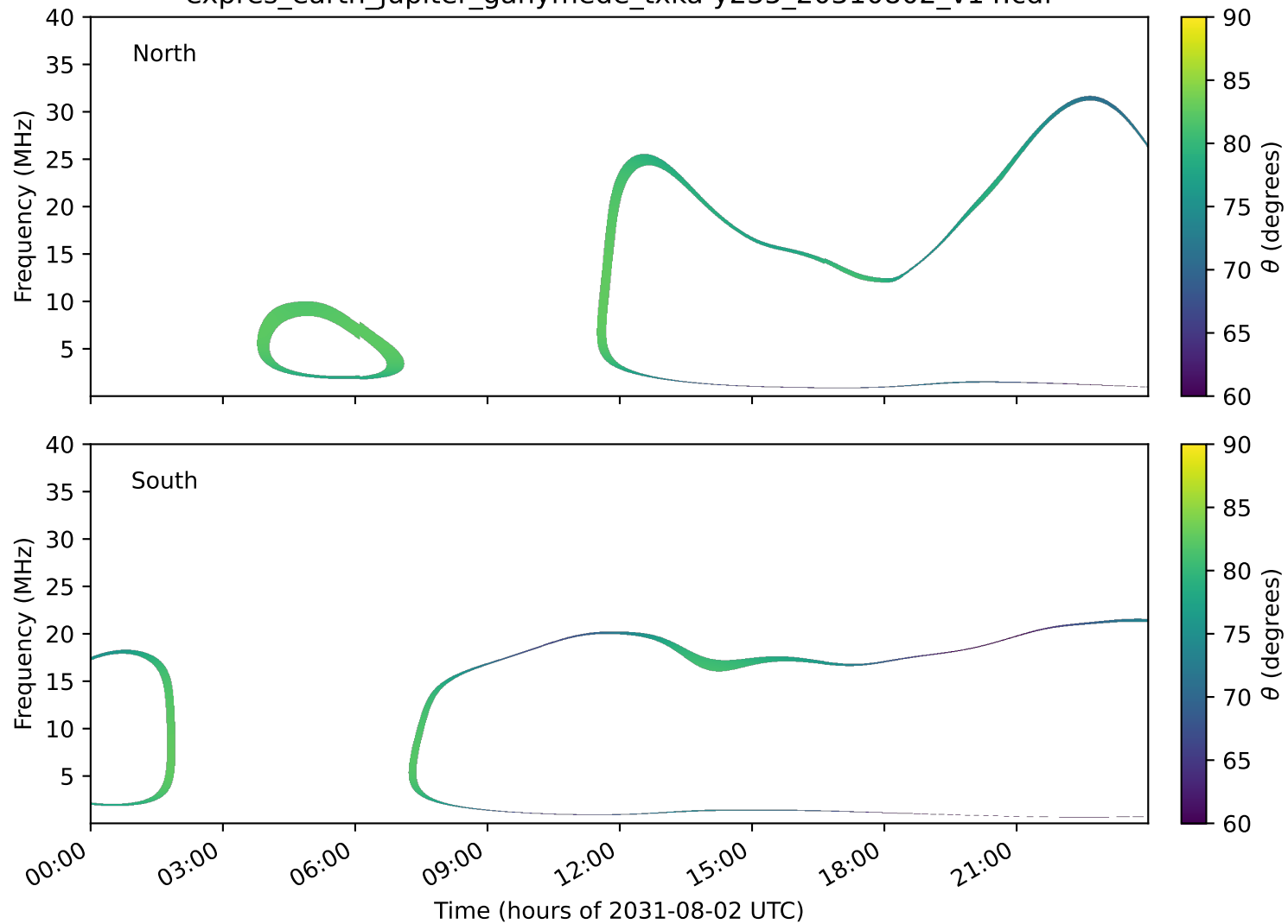
expres_earth_jupiter_ganymede_txka-y235_20310802_v14.cdf
