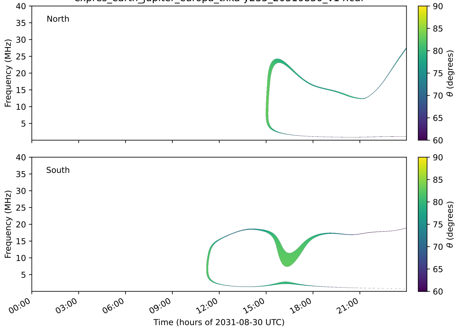
expres_earth_jupiter_europa_txka-y235_20310830_v14.cdf
