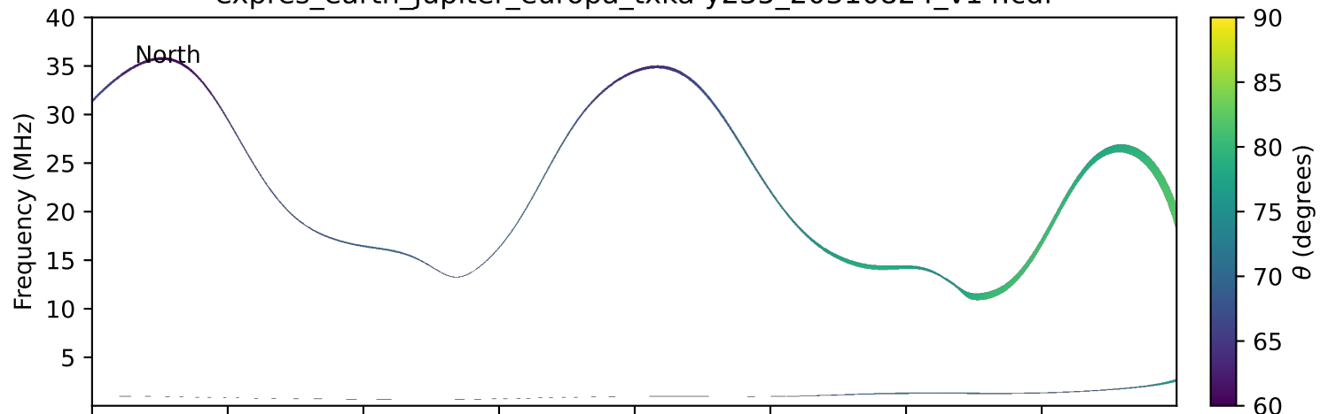
expres_earth_jupiter_europa_txka-y235_20310824_v14.cdf
