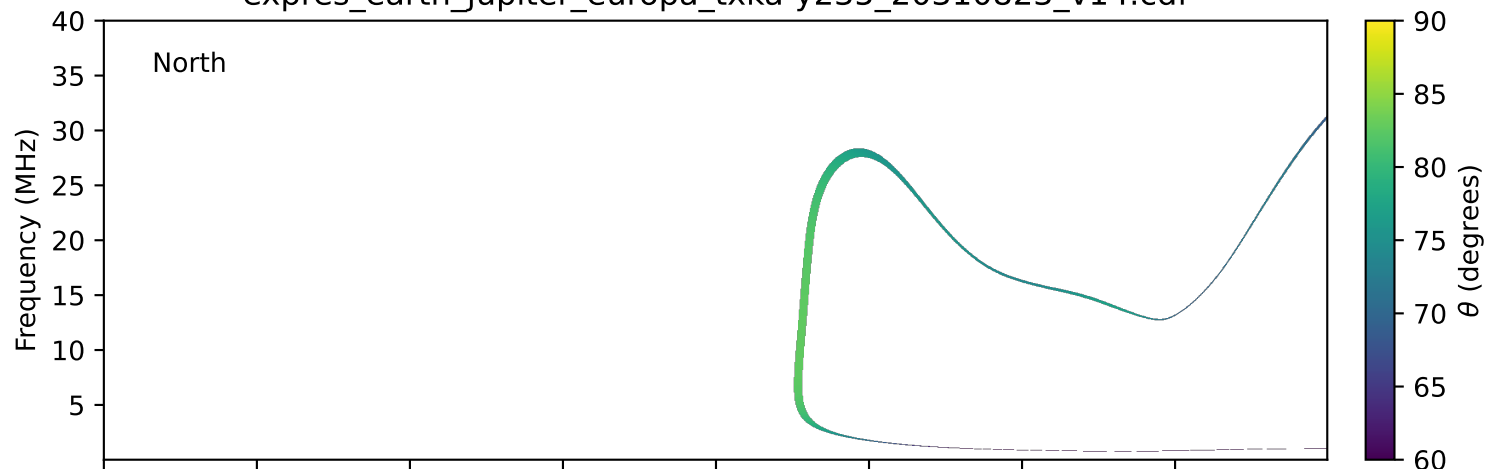
expres_earth_jupiter_europa_txka-y235_20310823_v14.cdf
