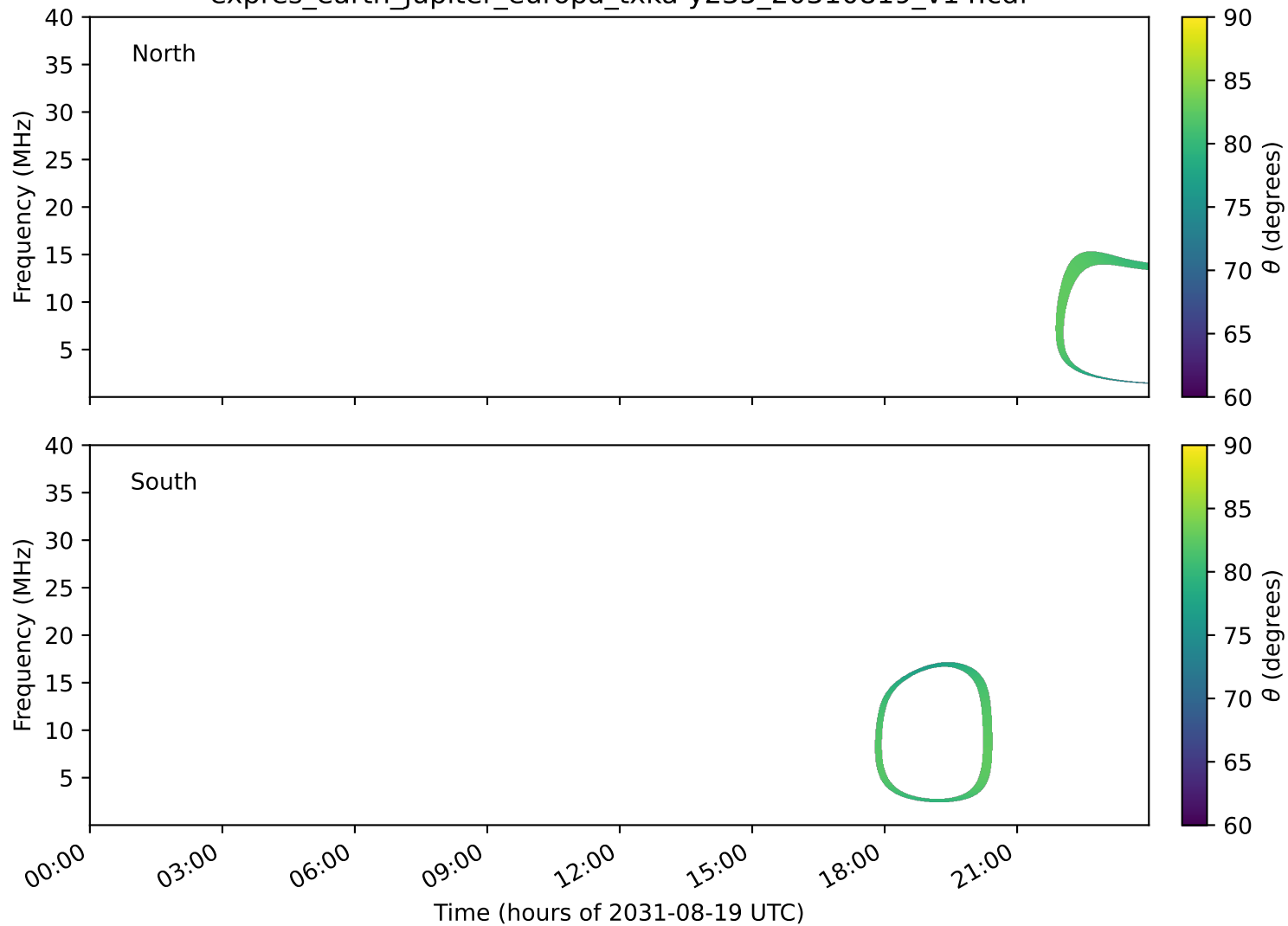
expres_earth_jupiter_europa_txka-y235_20310819_v14.cdf
