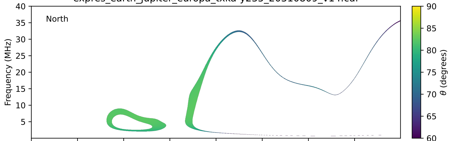
expres_earth_jupiter_europa_txka-y235_20310809_v14.cdf
