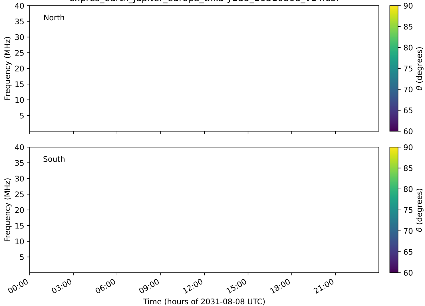
expres_earth_jupiter_europa_txka-y235_20310808_v14.cdf
