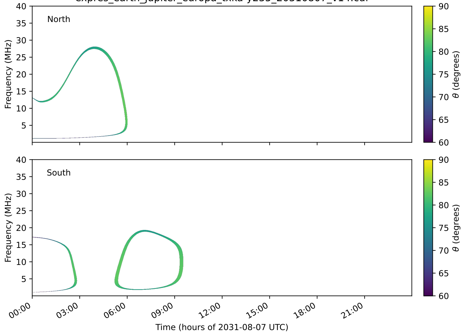
expres_earth_jupiter_europa_txka-y235_20310807_v14.cdf
