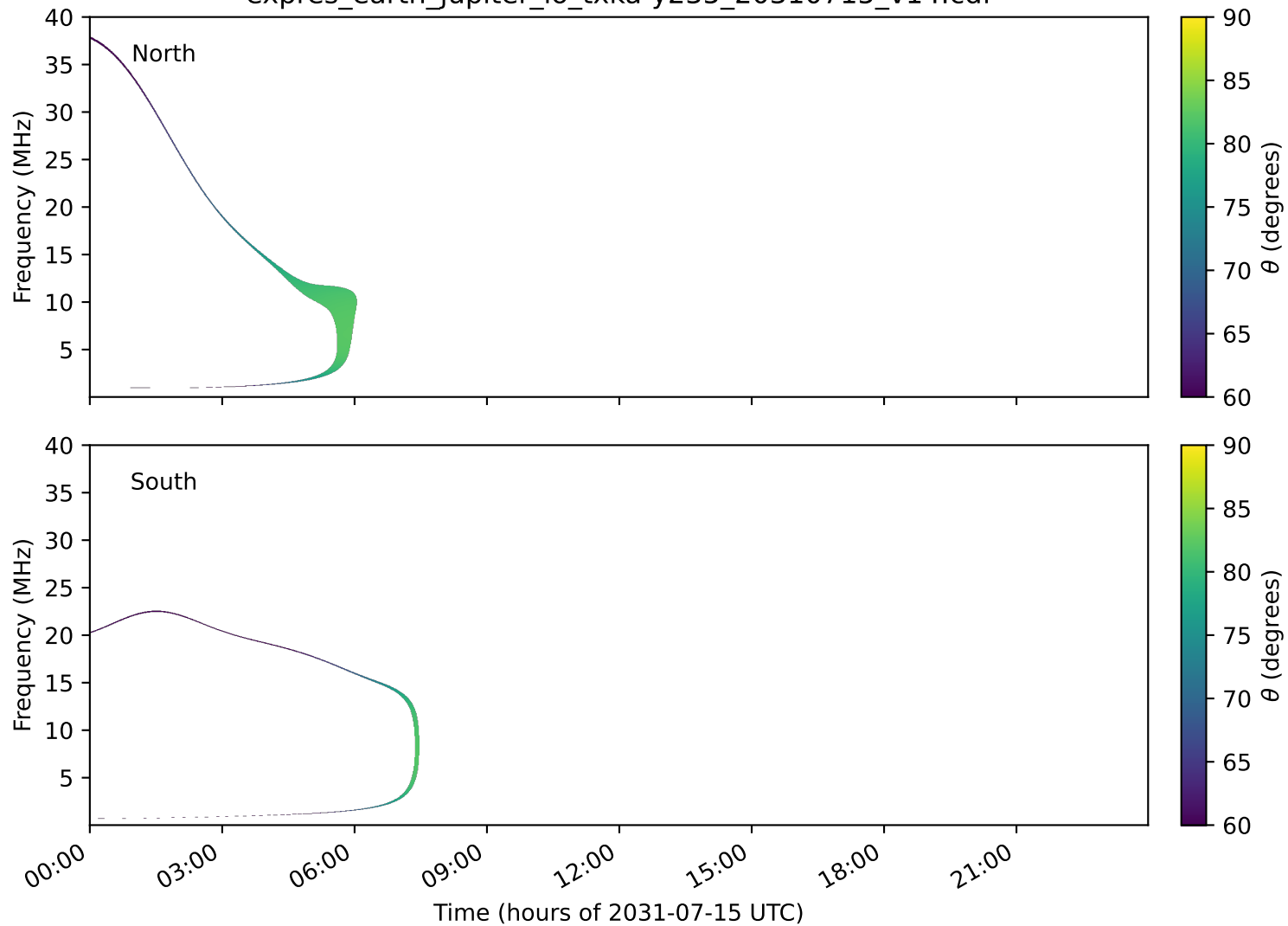
expres_earth_jupiter_io_txka-y235_20310715_v14.cdf
