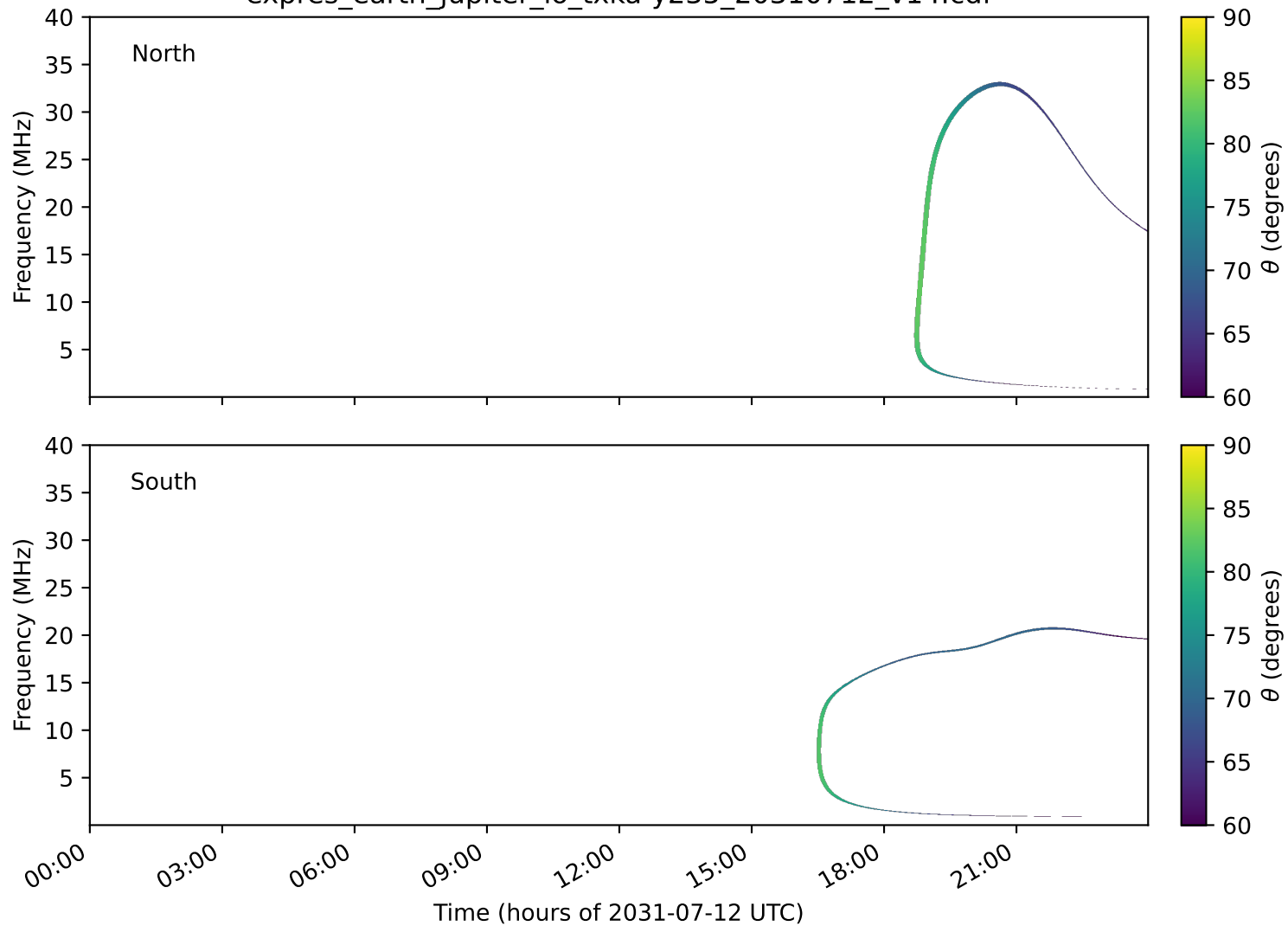
expres_earth_jupiter_io_txka-y235_20310712_v14.cdf
