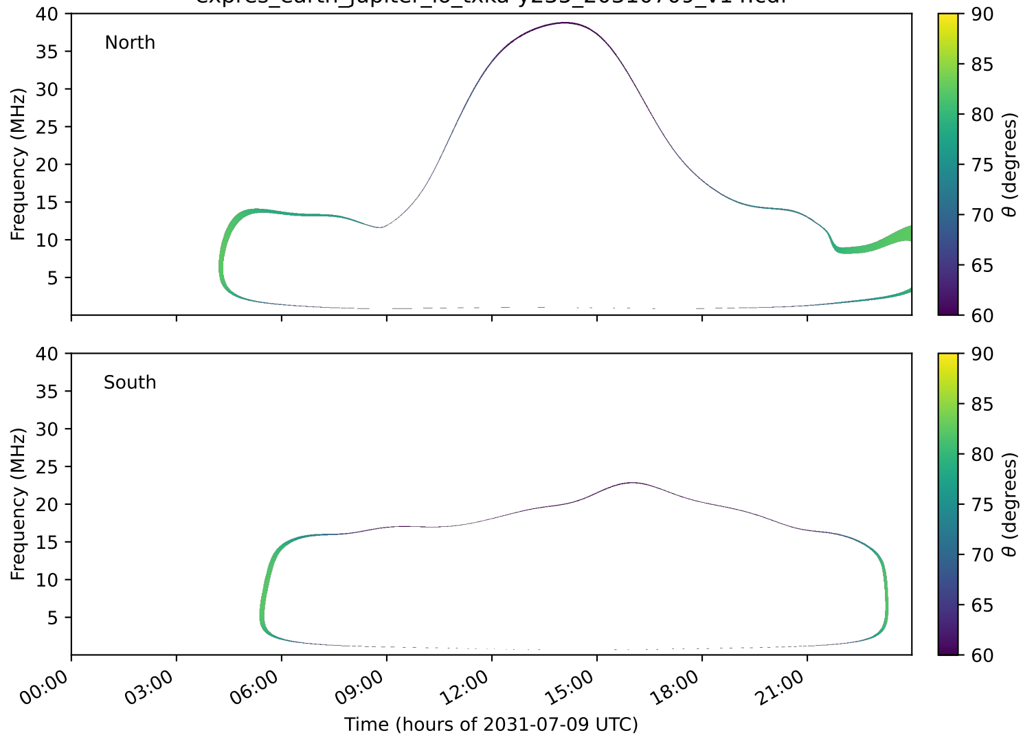
expres_earth_jupiter_io_txka-y235_20310709_v14.cdf
