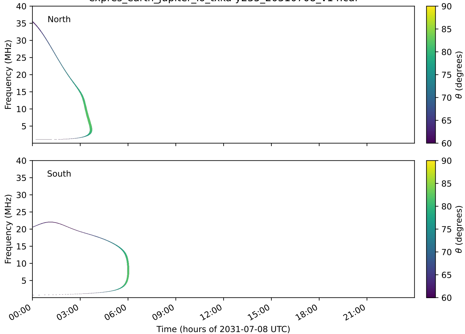
expres_earth_jupiter_io_txka-y235_20310708_v14.cdf
