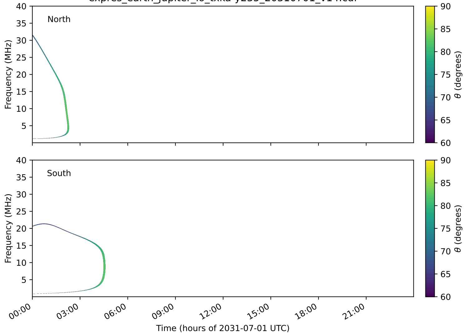
expres_earth_jupiter_io_txka-y235_20310701_v14.cdf
