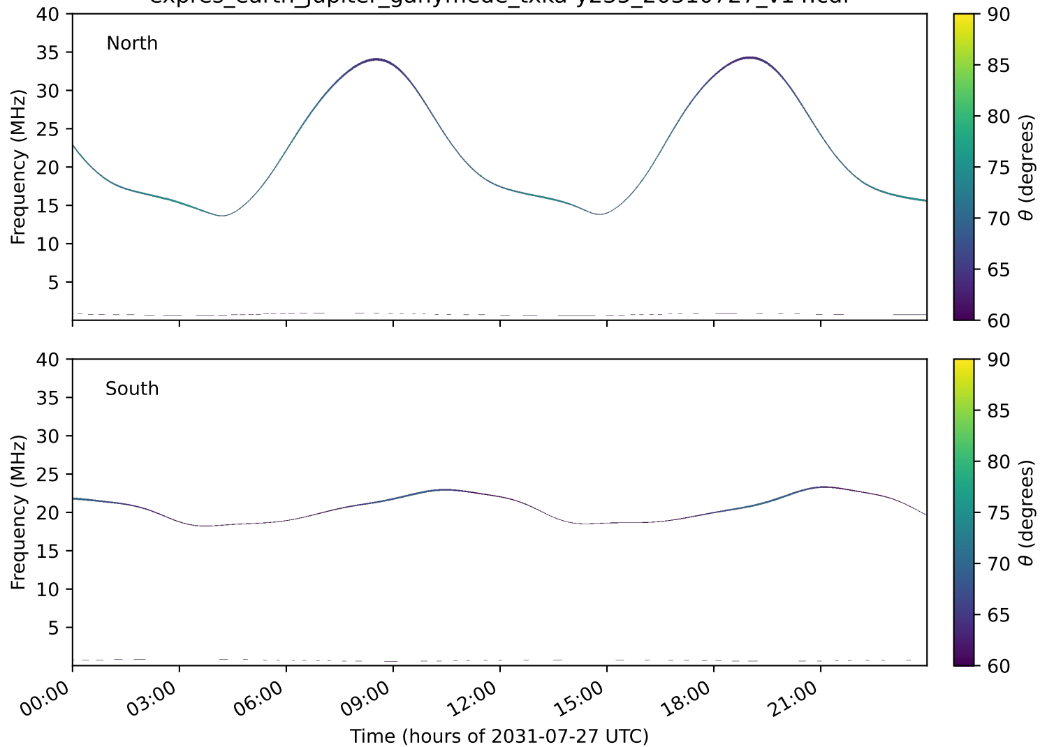
expres_earth_jupiter_ganymede_txka-y235_20310727_v14.cdf
