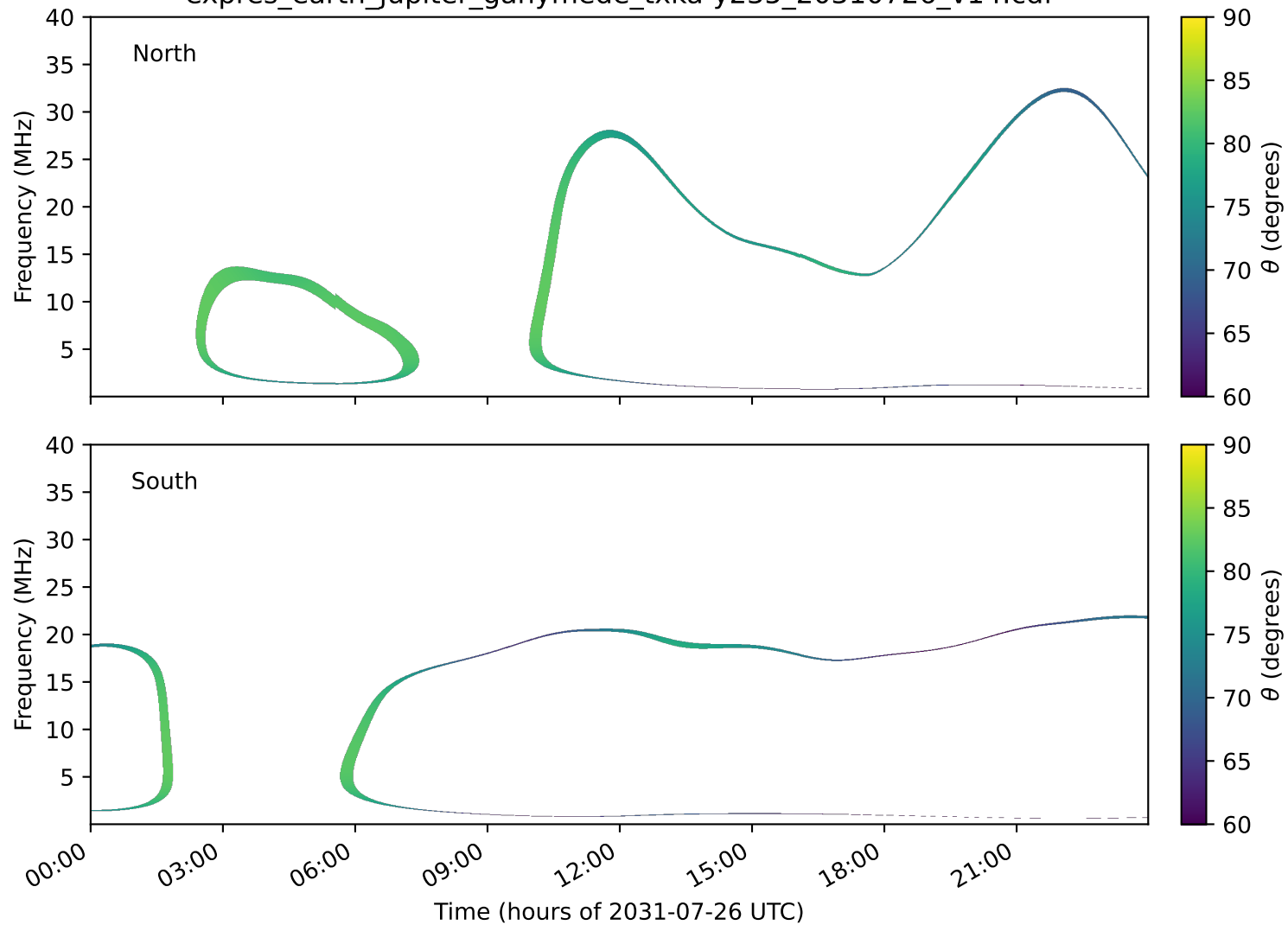
expres_earth_jupiter_ganymede_txka-y235_20310726_v14.cdf
