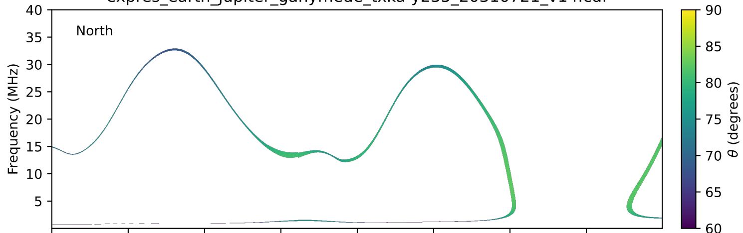
expres_earth_jupiter_ganymede_txka-y235_20310721_v14.cdf
