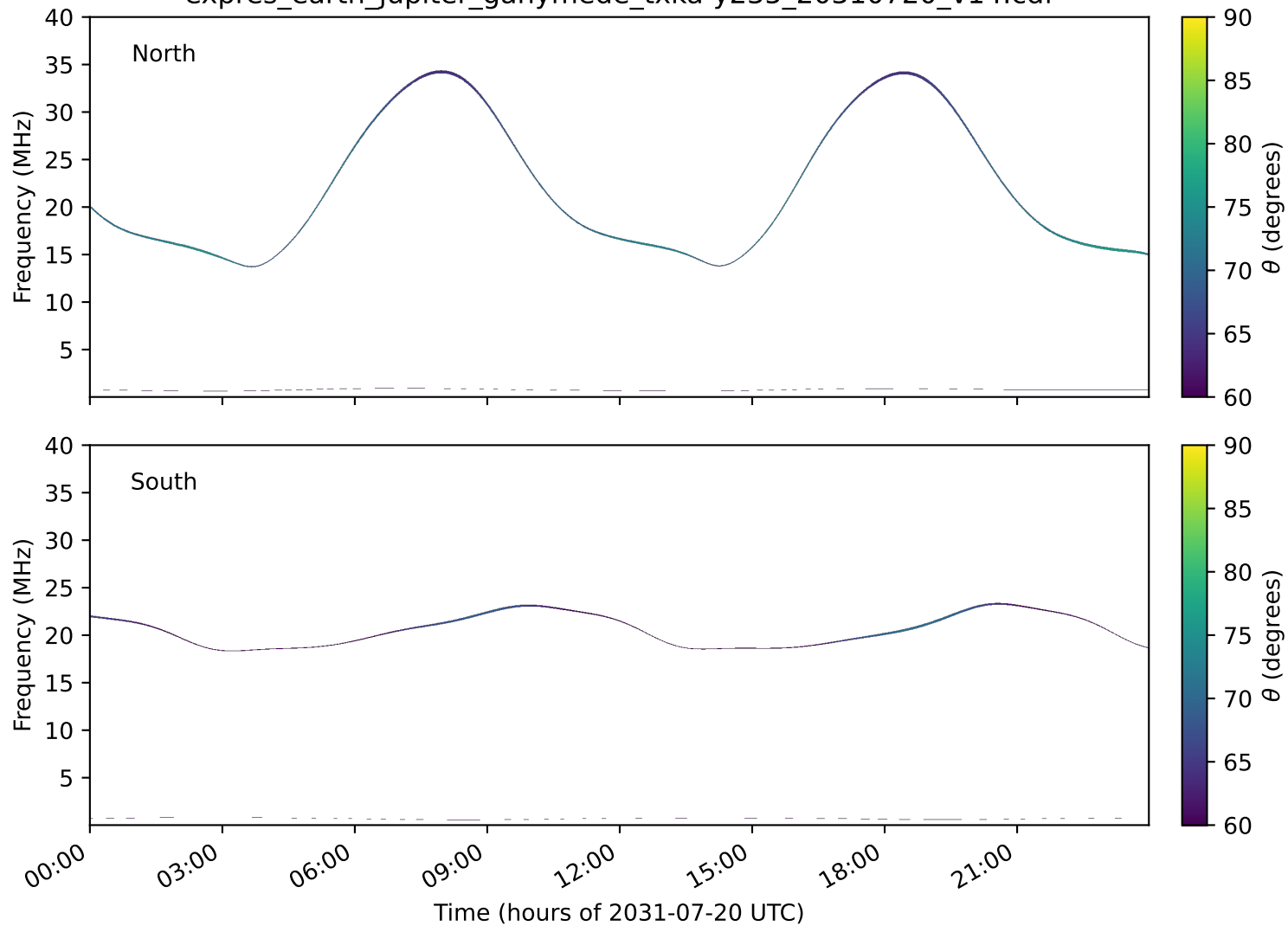
expres_earth_jupiter_ganymede_txka-y235_20310720_v14.cdf
