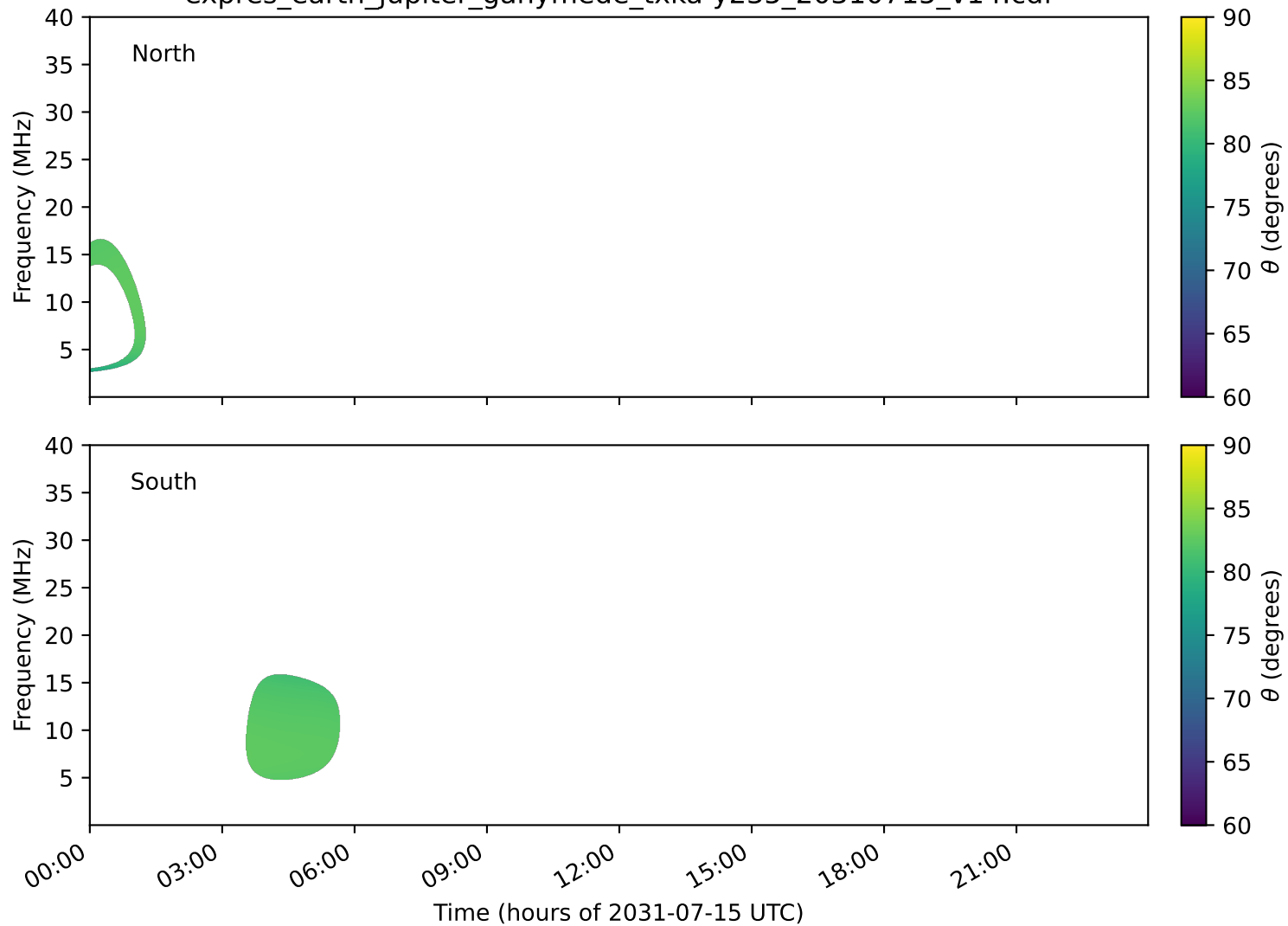
expres_earth_jupiter_ganymede_txka-y235_20310715_v14.cdf
