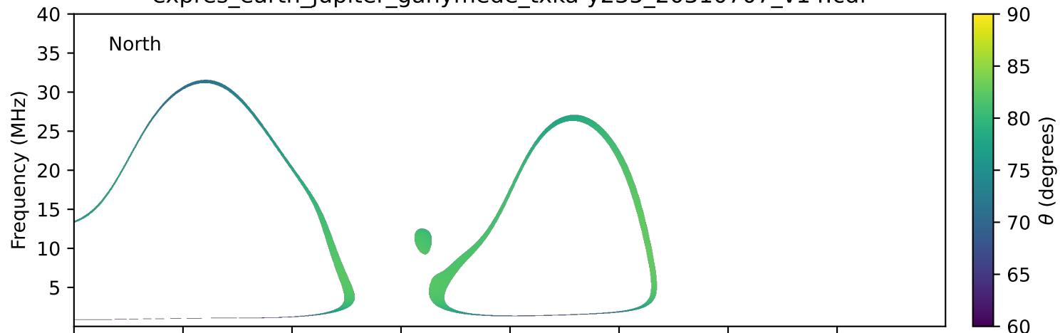
expres_earth_jupiter_ganymede_txka-y235_20310707_v14.cdf
