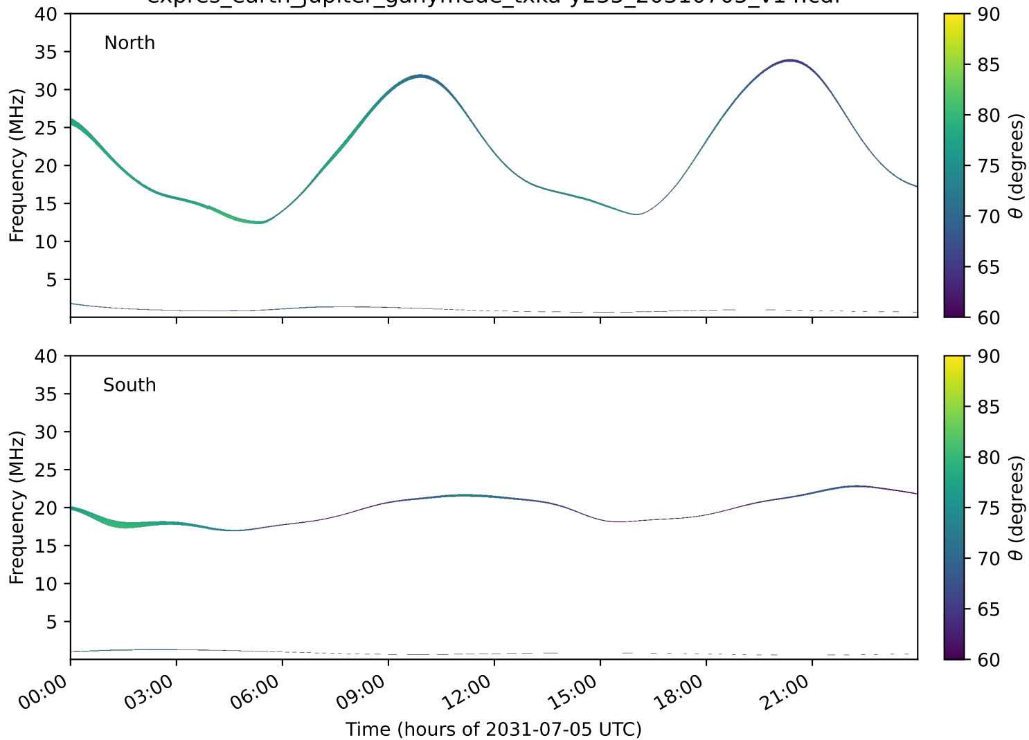
expres_earth_jupiter_ganymede_txka-y235_20310705_v14.cdf
