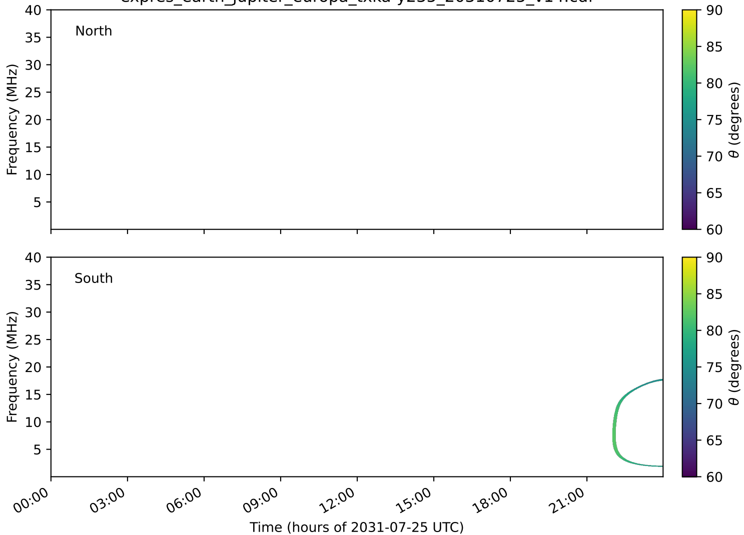
expres_earth_jupiter_europa_txka-y235_20310725_v14.cdf
