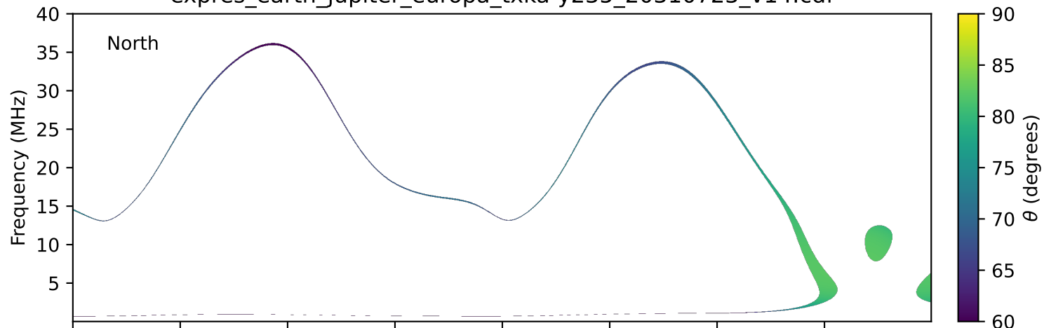
expres_earth_jupiter_europa_txka-y235_20310723_v14.cdf
