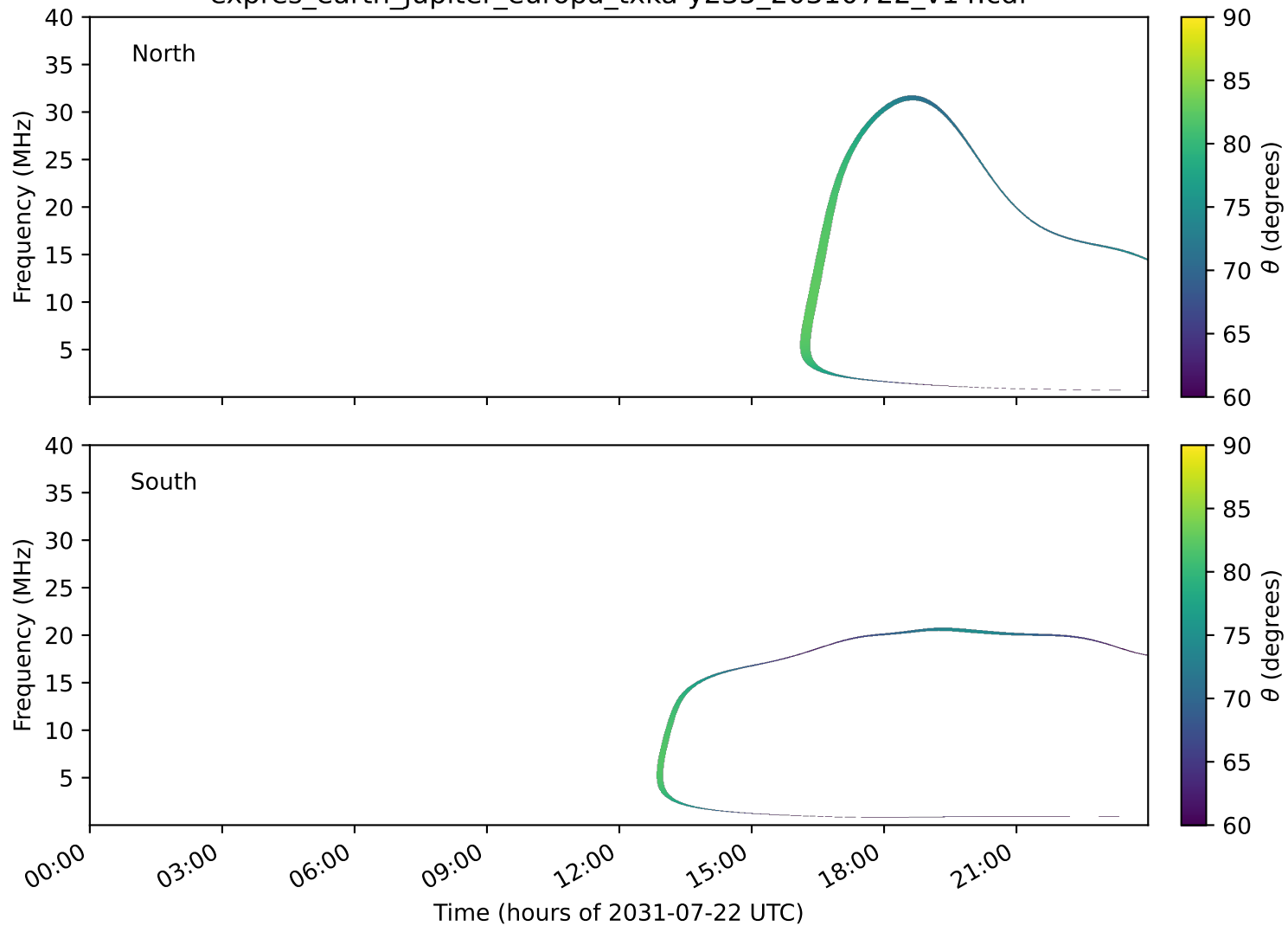
expres_earth_jupiter_europa_txka-y235_20310722_v14.cdf
