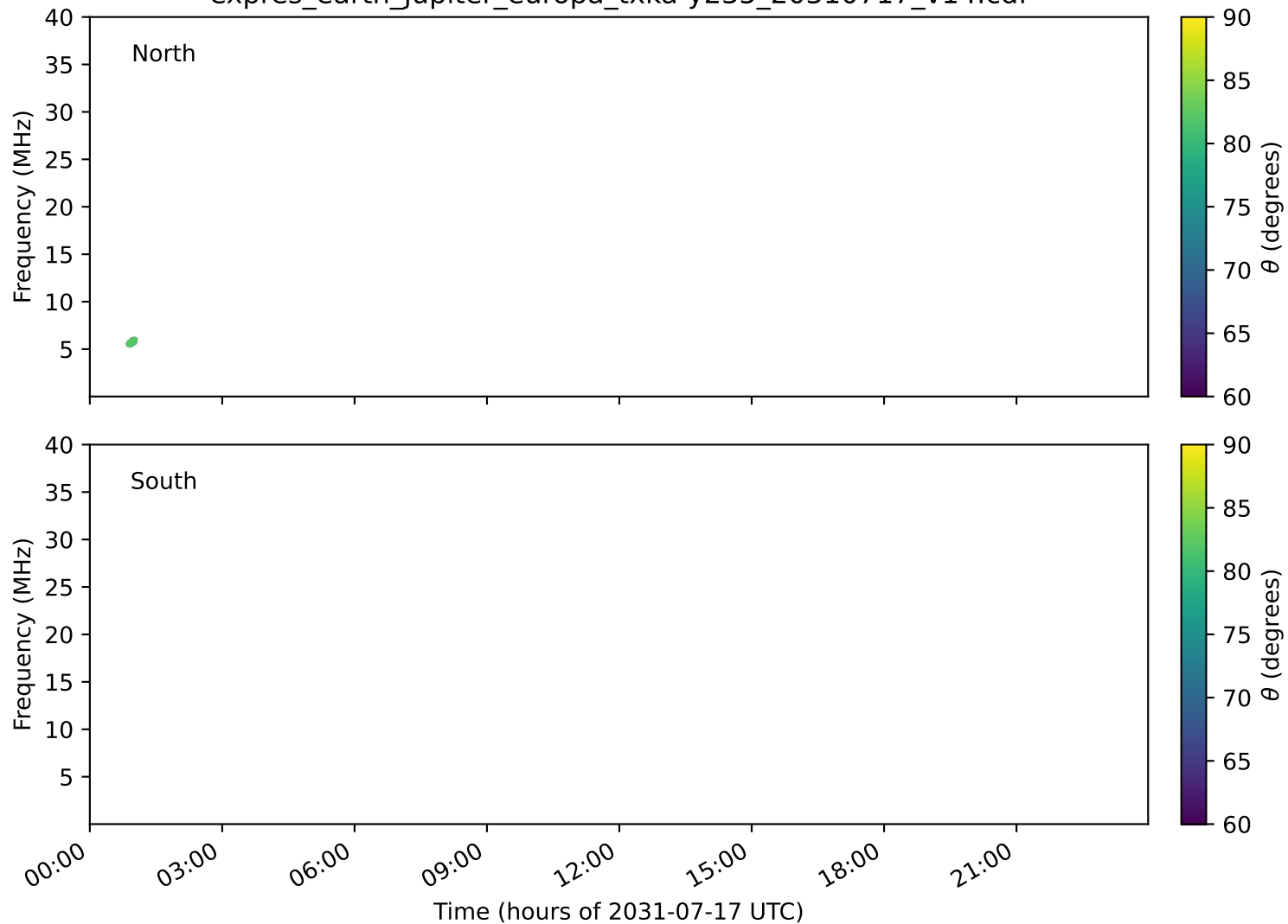
expres_earth_jupiter_europa_txka-y235_20310717_v14.cdf
