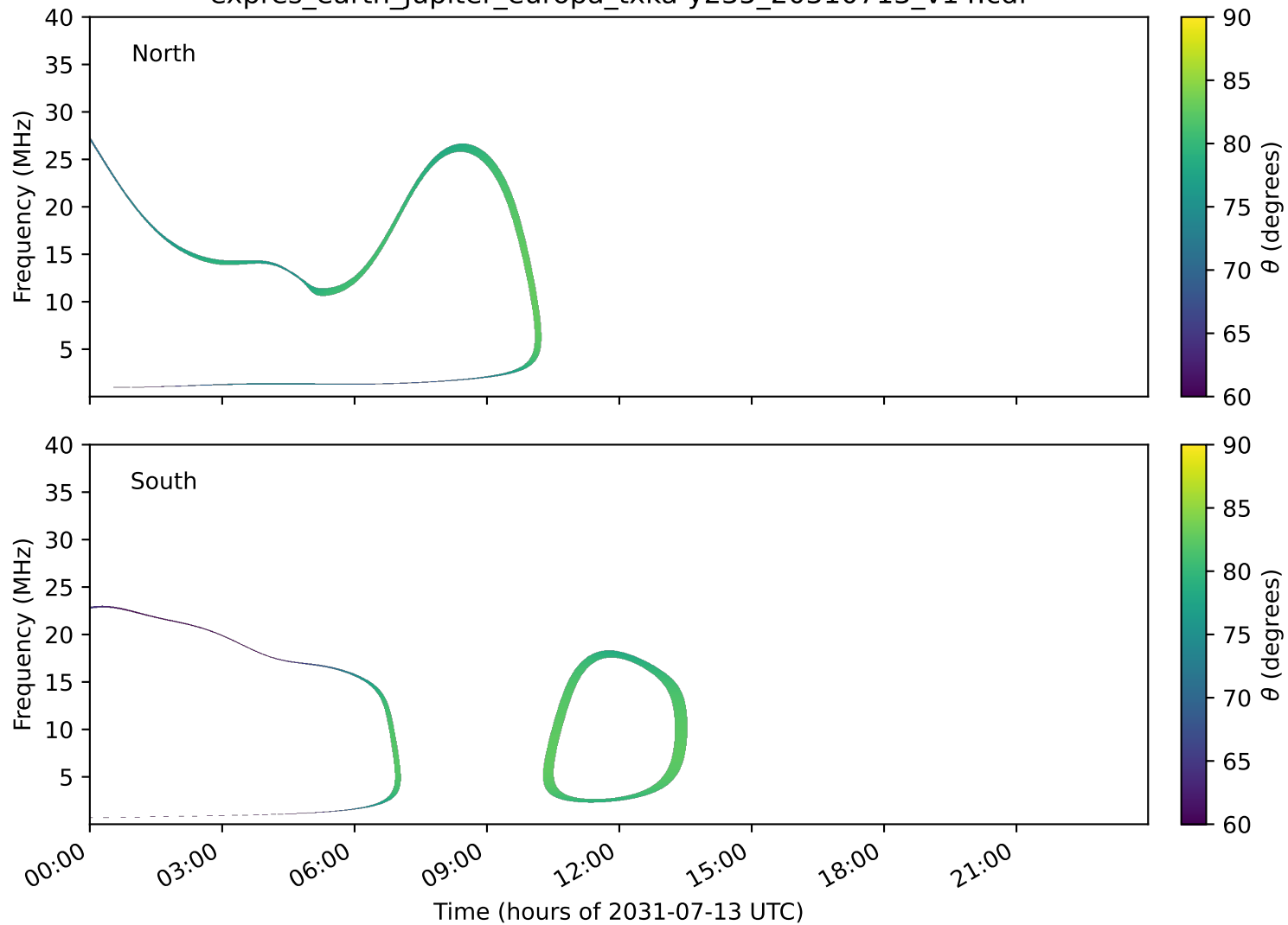
expres_earth_jupiter_europa_txka-y235_20310713_v14.cdf
