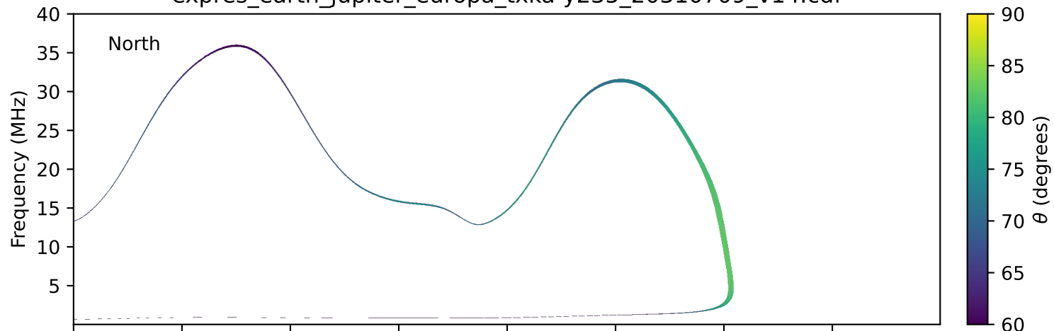
expres_earth_jupiter_europa_txka-y235_20310709_v14.cdf
