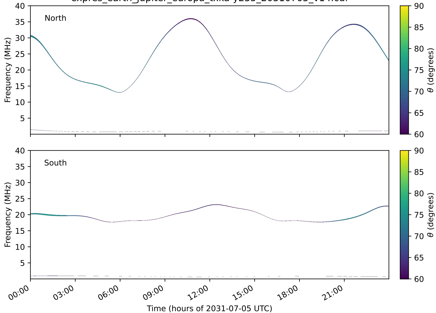
expres_earth_jupiter_europa_txka-y235_20310705_v14.cdf
