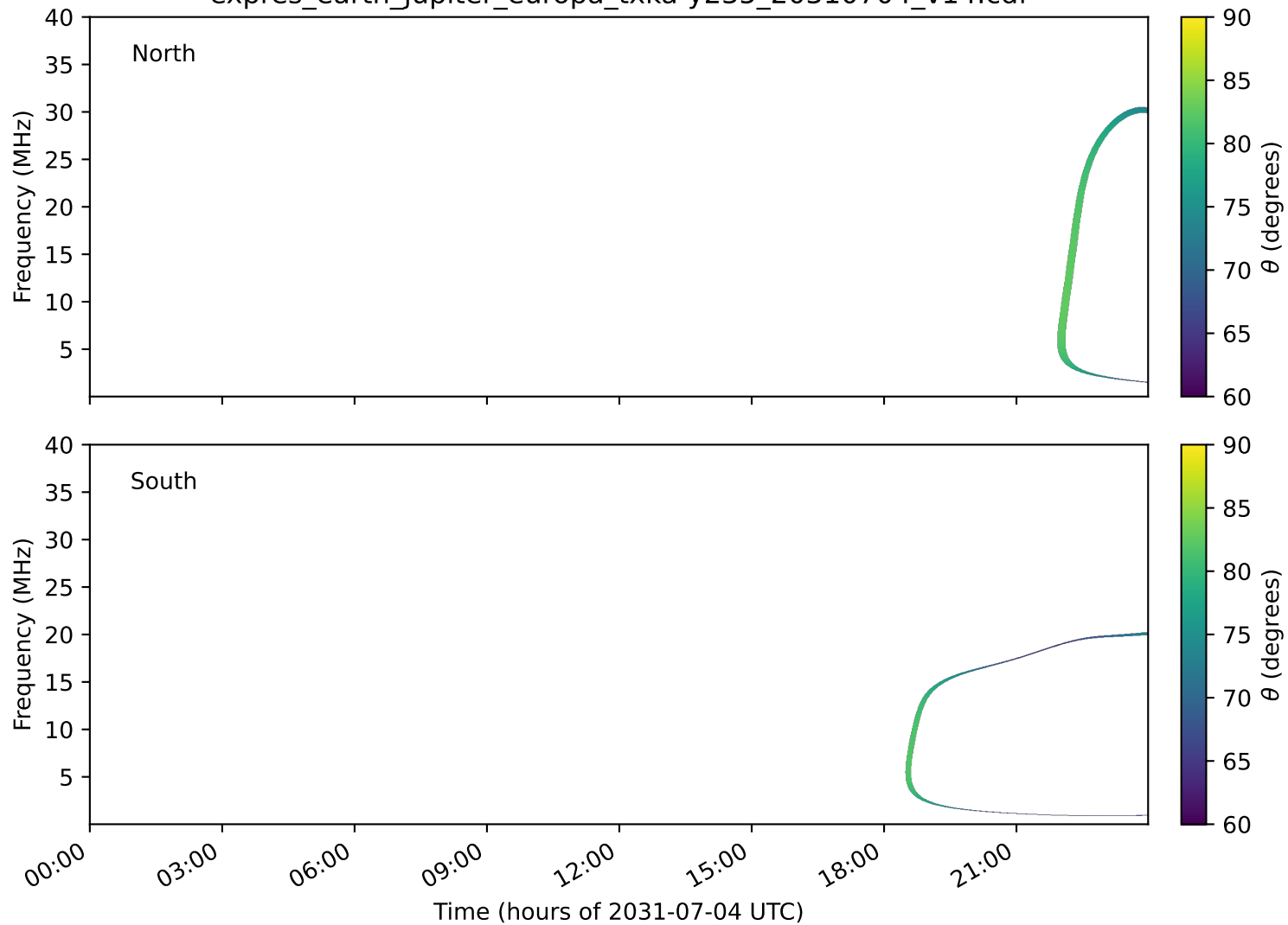
expres_earth_jupiter_europa_txka-y235_20310704_v14.cdf
