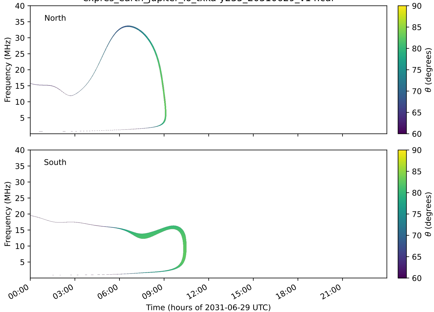
expres_earth_jupiter_io_txka-y235_20310629_v14.cdf
