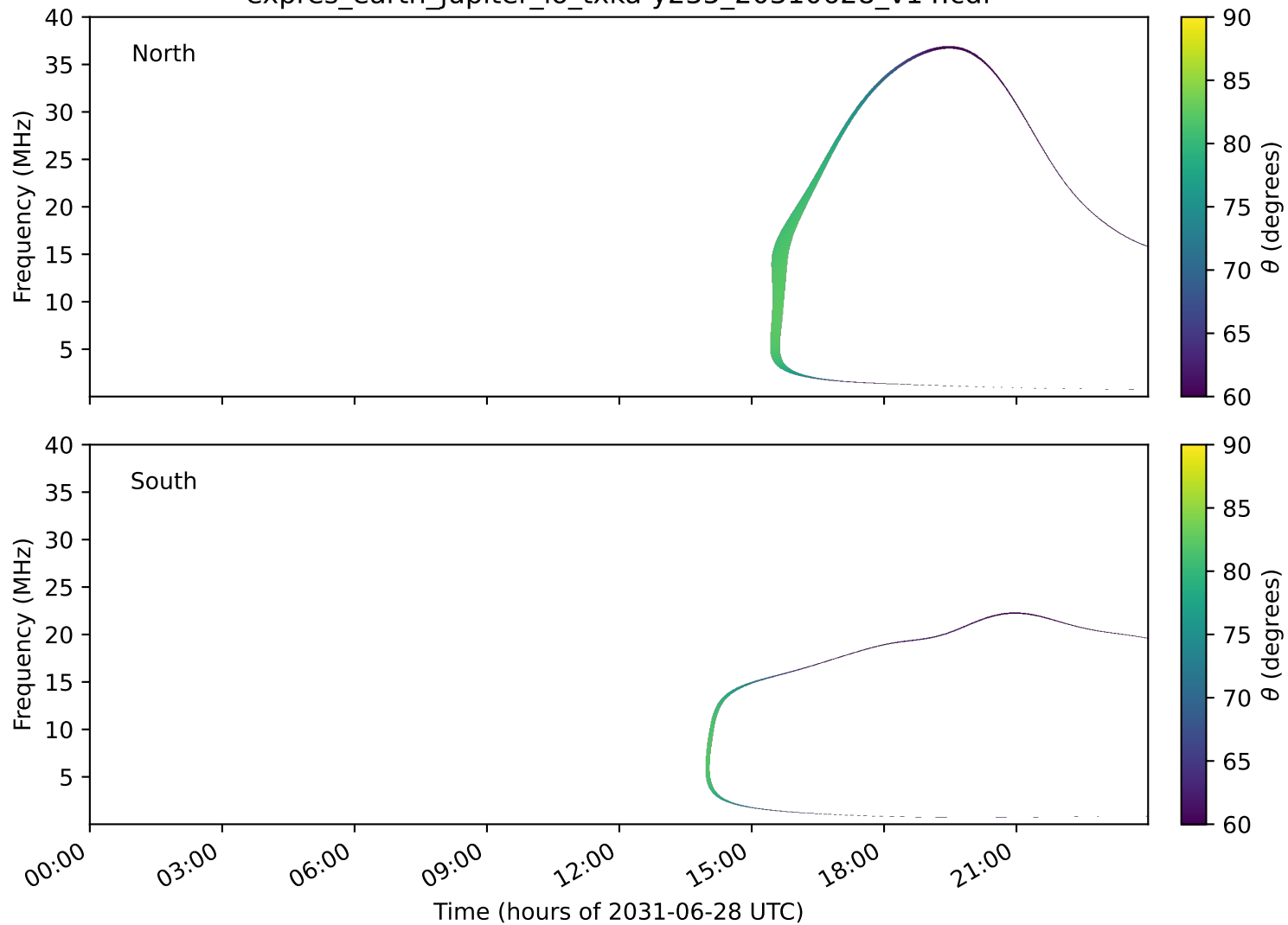
expres_earth_jupiter_io_txka-y235_20310628_v14.cdf
